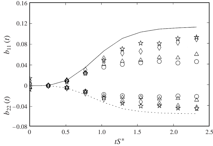
FIGURE 12. Anisotropy tensor b_{ij} of normalized stress r_{ij} . Solid line and upper set of symbols: 11-component; dashed line and lower set of symbols: 22-component. Stars: \Delta/\eta = 280 , rhombs: \Delta/\eta = 80 , triangles: \Delta/\eta = 40 , circles: \Delta/\eta = 20 ; lines: two-dimensional filtered RDT prediction.
